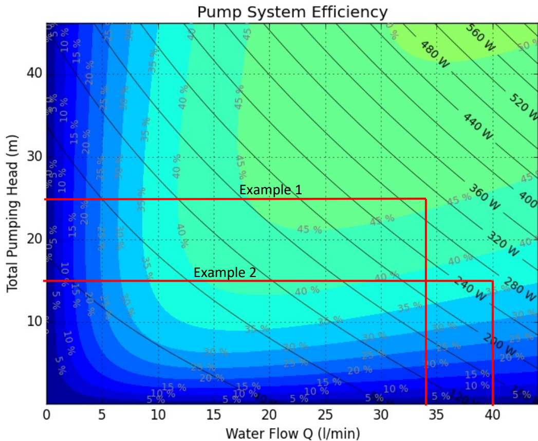
Water Flow in liter/min as a function of total pumping head and maximum solar power
